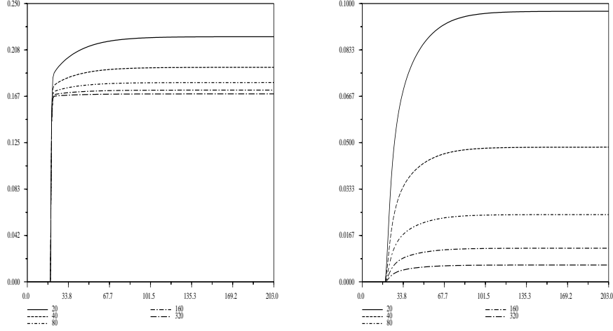
Figure 2: The focalization coefficient against the number of iterations in the Boltzmann-Lorentz case (left), and in the Fokker-Planck-Lorentz case (right)
