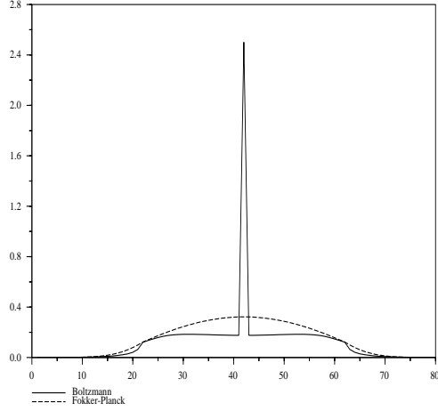
Figure 1: The outgoing profile f(x = 1, \cdot, t = 0.5) versus the velocity angle \theta in the Boltzmann and Fokker-Planck case ( N_\theta = 80 )
