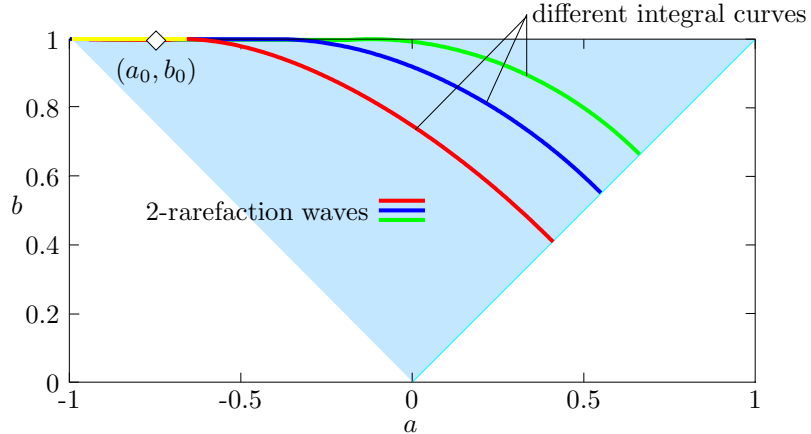
Figure 4: 2-rarefaction waves through (a_0, b_0) (the shaded region represents the set of Cauchy data considered in proposition 4).
